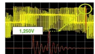
E=650V, cable=100m
